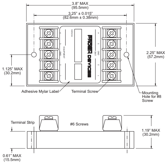
TEL50E CASE OUTLINE
